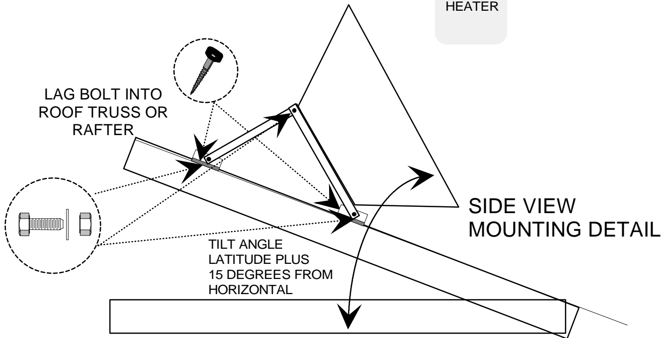
COLLECTOR AND TANK IN ONE UNIT
