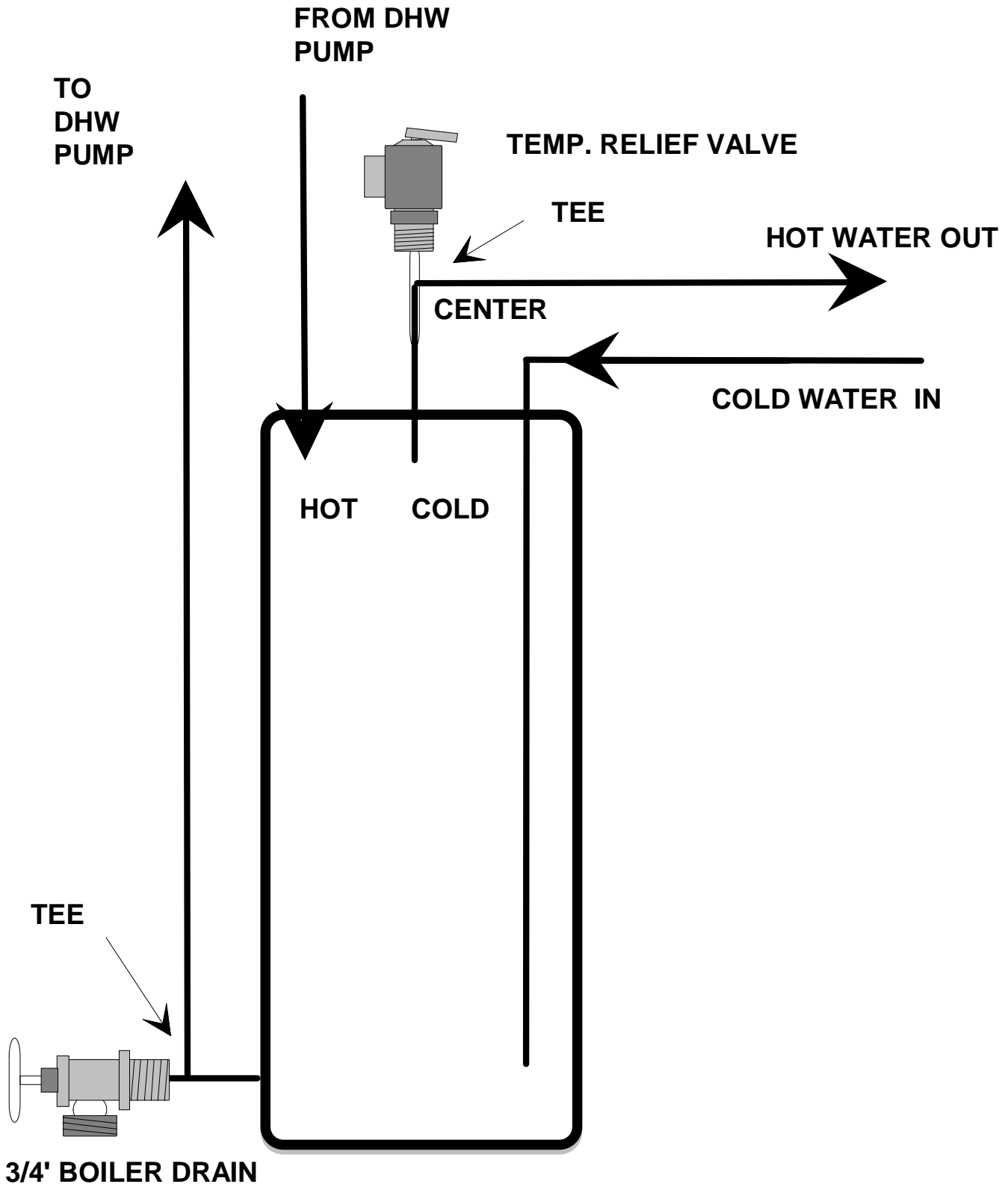
PIPING A WATER HEATER AS A SOLAR STORAGE TANK
